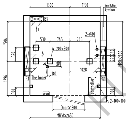
Machine room plan/1:60
