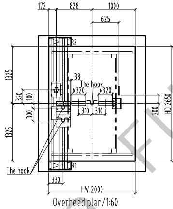
Overhead plan/1:60
