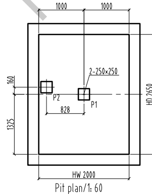
Pit plan/1:60
