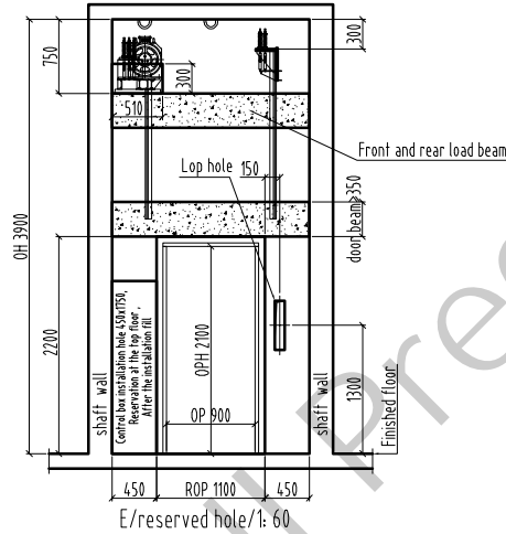
E/reserved hole/1:60
