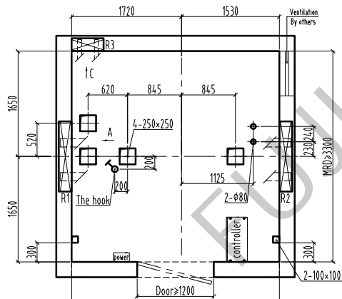
Machine room plan/1:60
