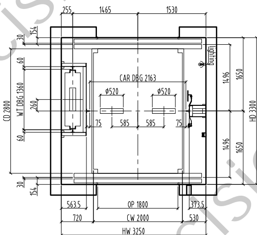
Hoistway plan/1:60
