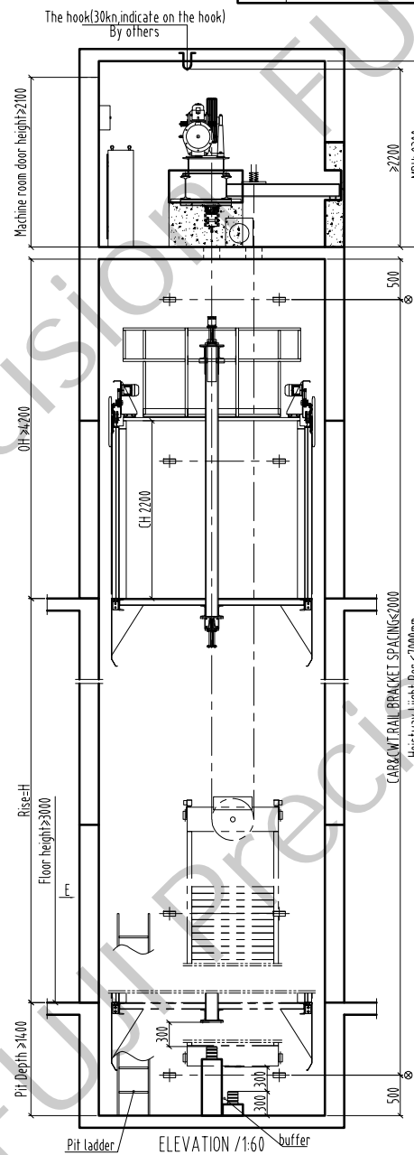
ELEVATION /1:60
