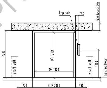
E/ reserved hole/1: 60
