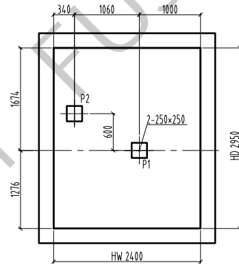
Pit plan/1: 60
