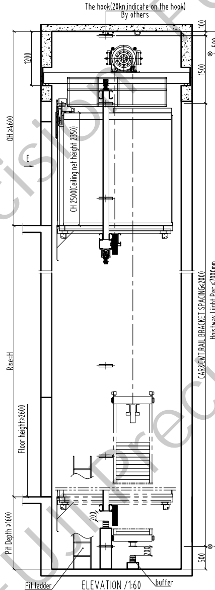
Pit ladder ELEVATION /1:60 buffer
