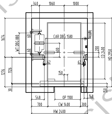
Hoistway plan/1:60
