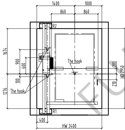
Overhead plan/1:60
