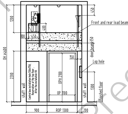
E/reserved hole/1: 60
